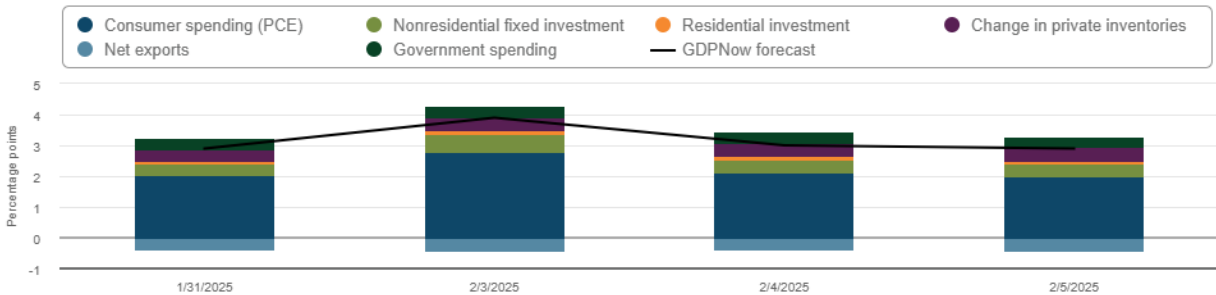
Subcomponent contributions to GDPNow real GDP growth forecasts
